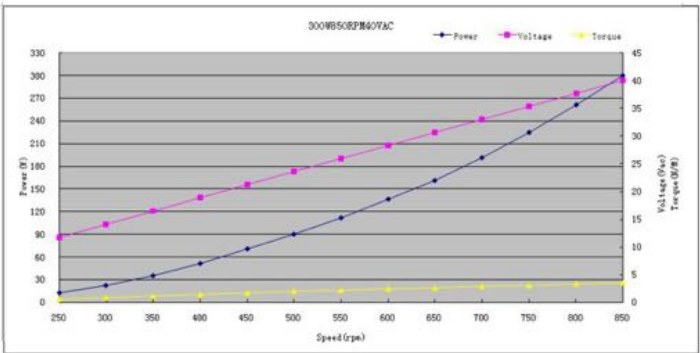
Power curve by Aeroleaf (without petal) Voltage / Power / Rotation speed
